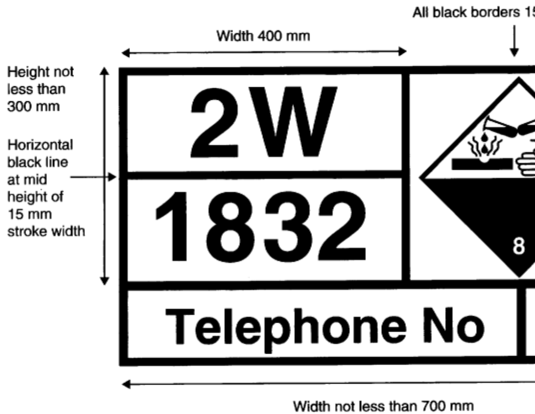
Figure 2 Hazard warning panel
